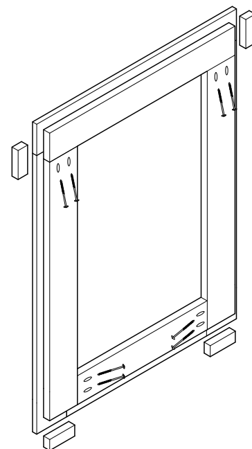
POCKET SCREWS/SQUARE CORNERS (BACK VIEW)
