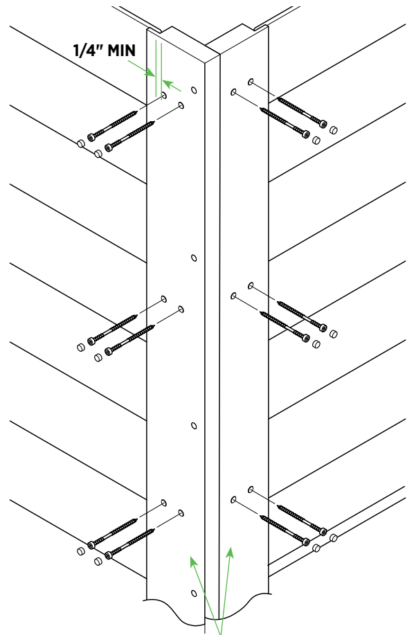
ATTACH TO WALLS EVERY 16" ON BOTH SURFACES. FASTENERS MUST NOT BE CLOSER THAN 1/4" FROM THE END OF THE POCKET.
